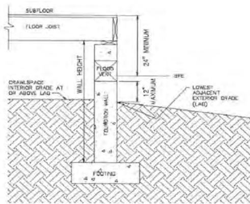
Figure 02-1: Preferred Crawl Space Construction 73
