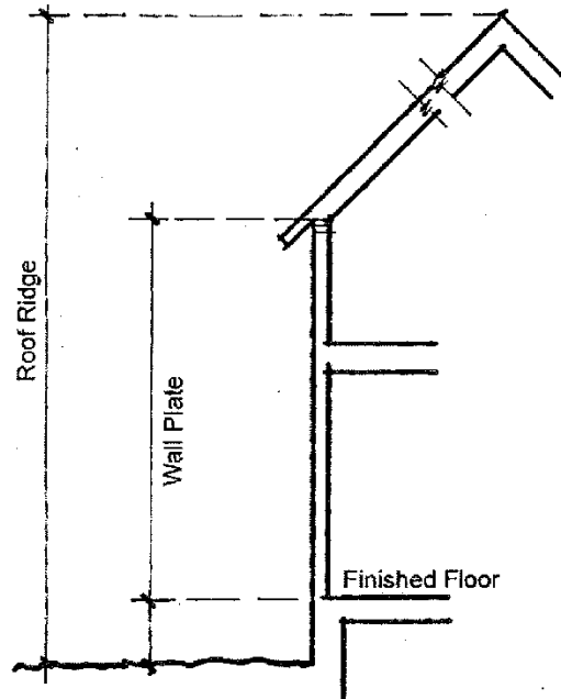
Figure 02-4: Plate Height at Minimum Setback 85
