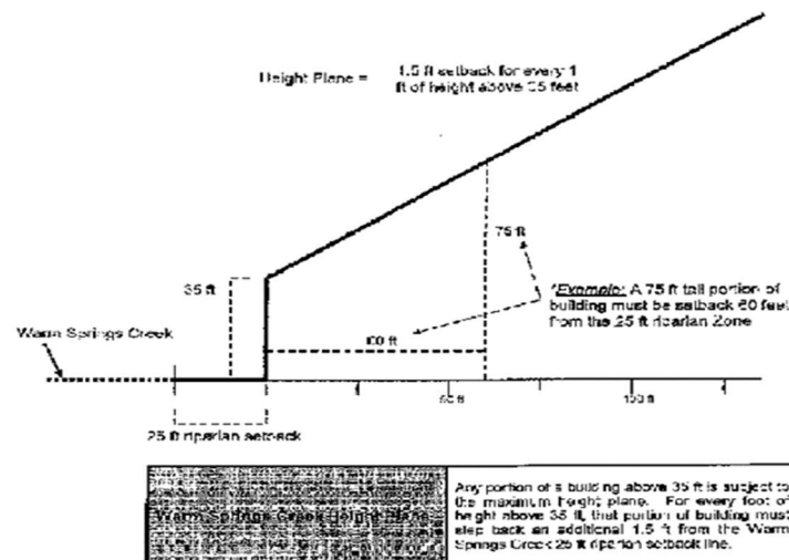
Figure 02-5: Height Plane Calculation 87
