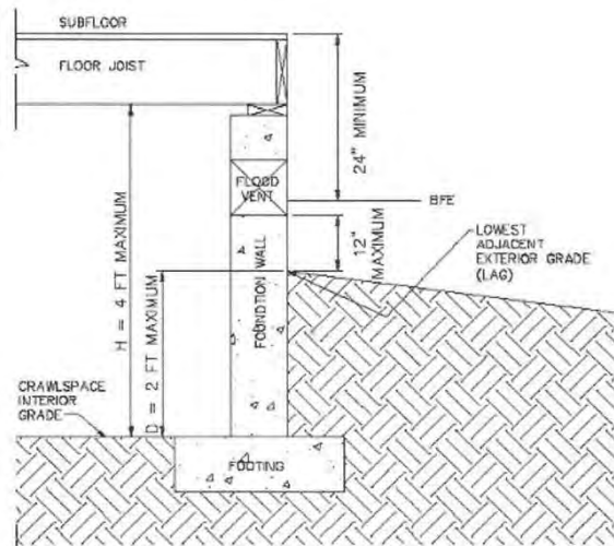
Figure 02-2: Below Grade Crawl Space Construction 74
