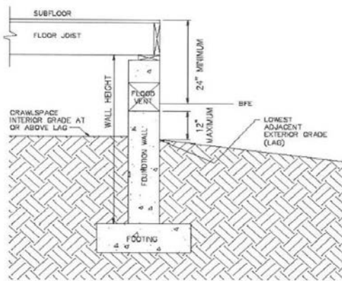
Figure 02-1: Preferred Crawl Space Construction 70
