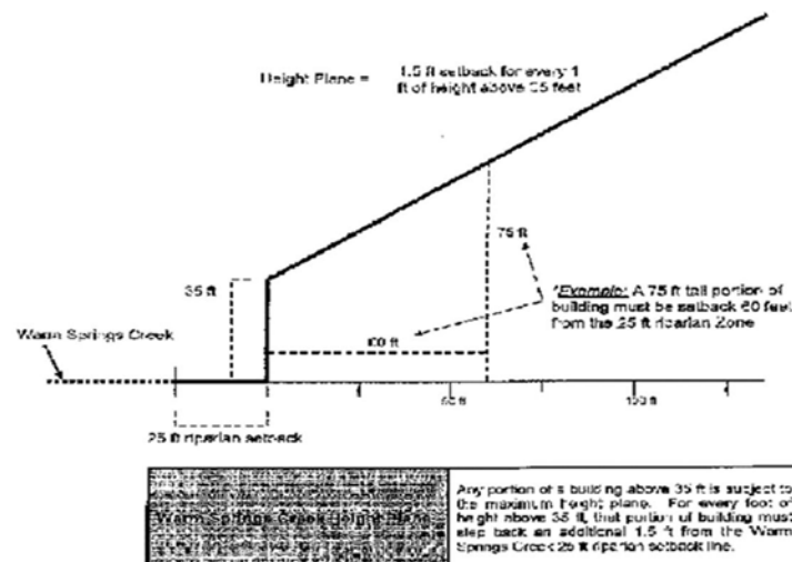
Figure 02-5: Height Plane Calculation 84
