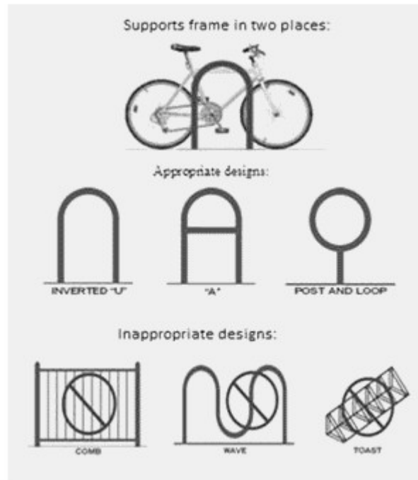
Figure 04-1: Bicycle Rack Designs 140
