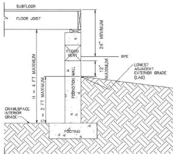
Figure 02-2: Below Grade Crawl Space Construction 71
