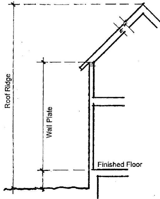
Figure 02-4: Plate Height at Minimum Setback 82
